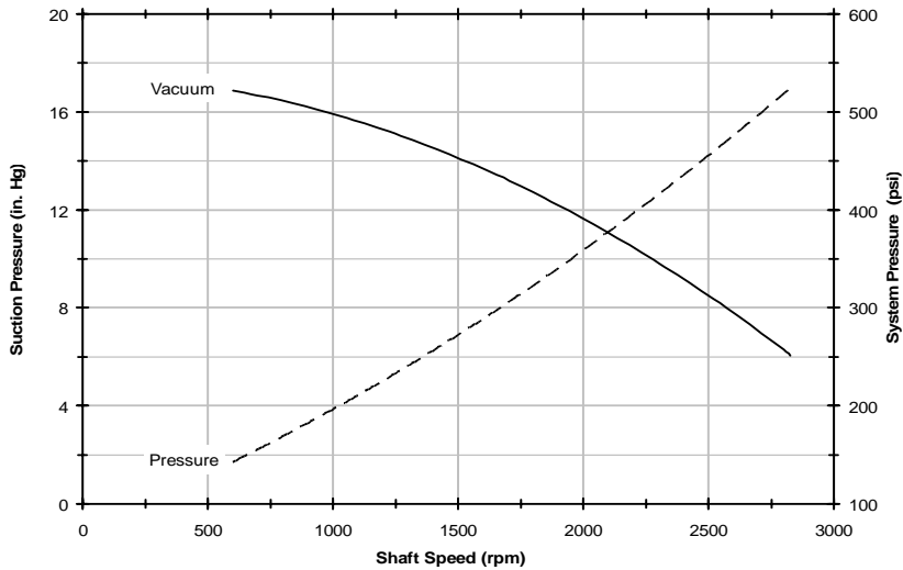
PVX580 pump inlet characteristics based on ISO 32 Oil @ 115°F
