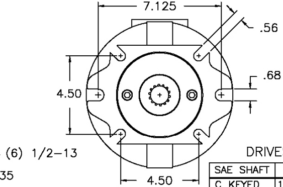
SAE "C" 4 BOLT MOUNTING FLANGE
