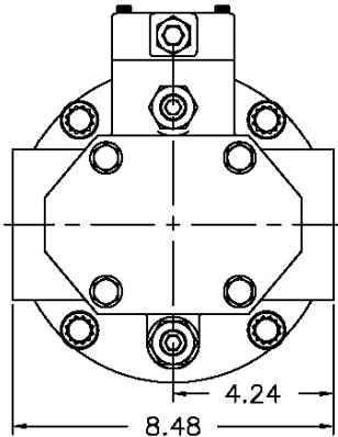
SAE "B" 2 & 4 BOLT MOUNTING FLANGE
