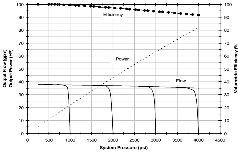
PVX580 pump performance @ 1750 rpm using ISO 32 oil at 115° F
