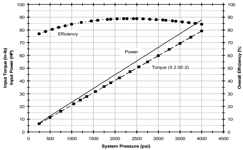
PVX580 pump input power curves @ 1750 rpm using ISO 32 oil at 115° F
