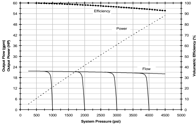
PVX348 pump performance @ 1750 rpm using ISO 32 oil at 115° F
