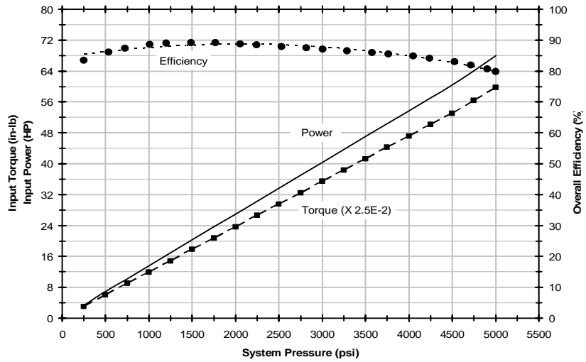
PVX348 pump input power curves @ 1750 rpm using ISO 32 oil at 115° F
