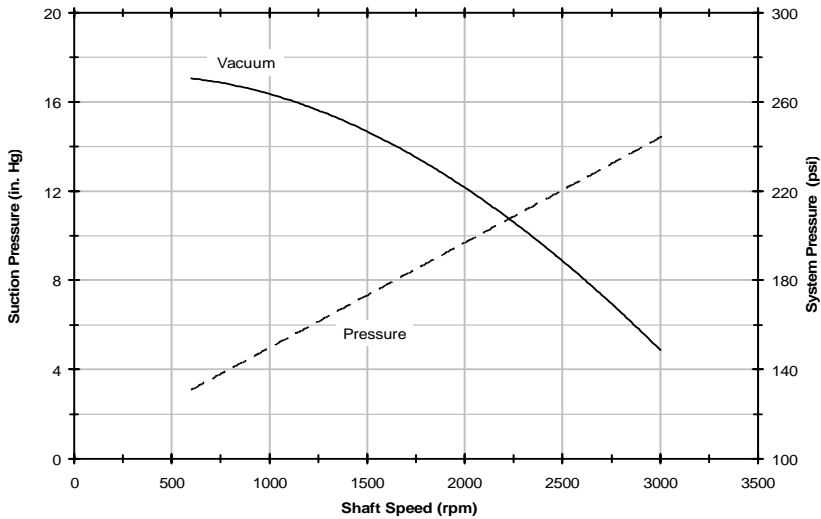
PVX348 pump inlet characteristics based on ISO 32 Oil @ 115°F
