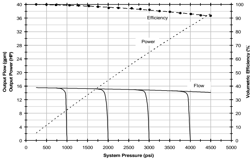
PVX232 pump performance @ 1750 rpm using ISO 32 oil at 115° F
