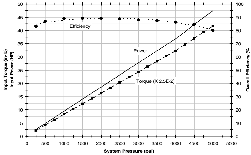
PVX232 pump input power curves @ 1750 rpm using ISO 32 oil at 115° F
