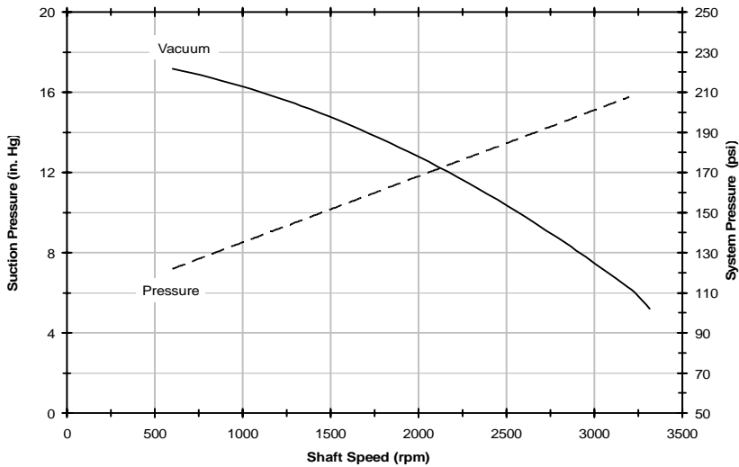
PVX232 pump inlet characteristics based on ISO 32 Oil @ 115°F
